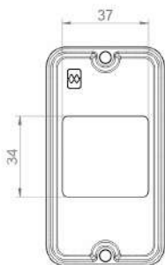
TAMPA P/ 2 INTERRUPTORES HORIZONTAIS 1/2" E 3/4"
