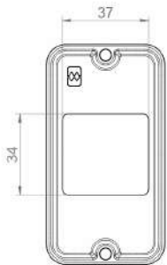
TAMPA P/ 2 INTERRUPTORES HORIZONTAIS 1/2" E 3/4"
